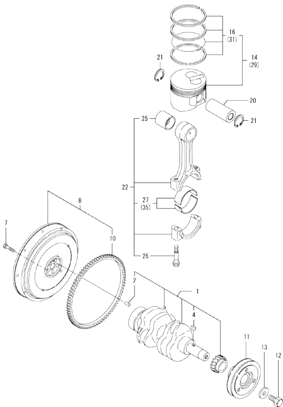
Fig.8. CRANKSHAFT & PISTON
