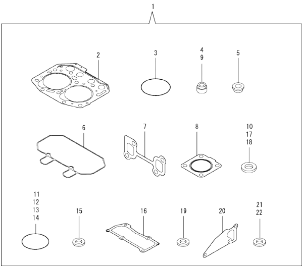
Fig.17. GASKET SET
